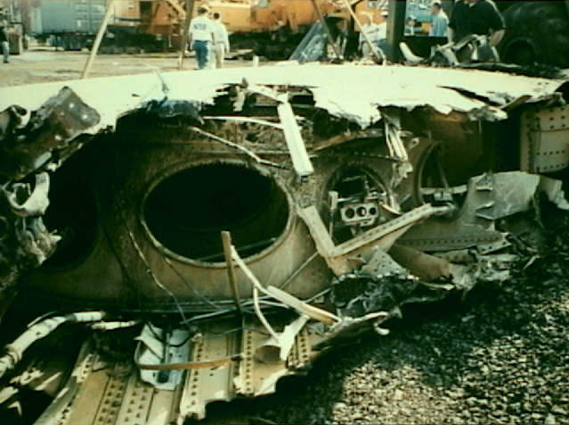
Structures 7 - Photo. 3. View looking at inboard right wing near WS 264.
