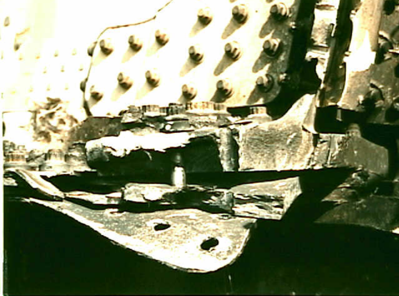
Structures 7 - Photo. 12 - View of upper rear spar cap fracture face at inboard right wing root side of body.
