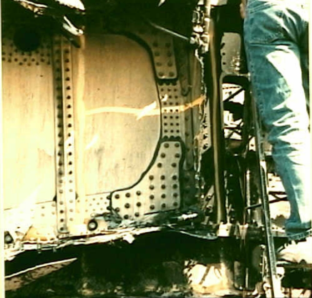
Structures 7 - Photo. 11 - View of fractured inboard right wing root at side of body.
