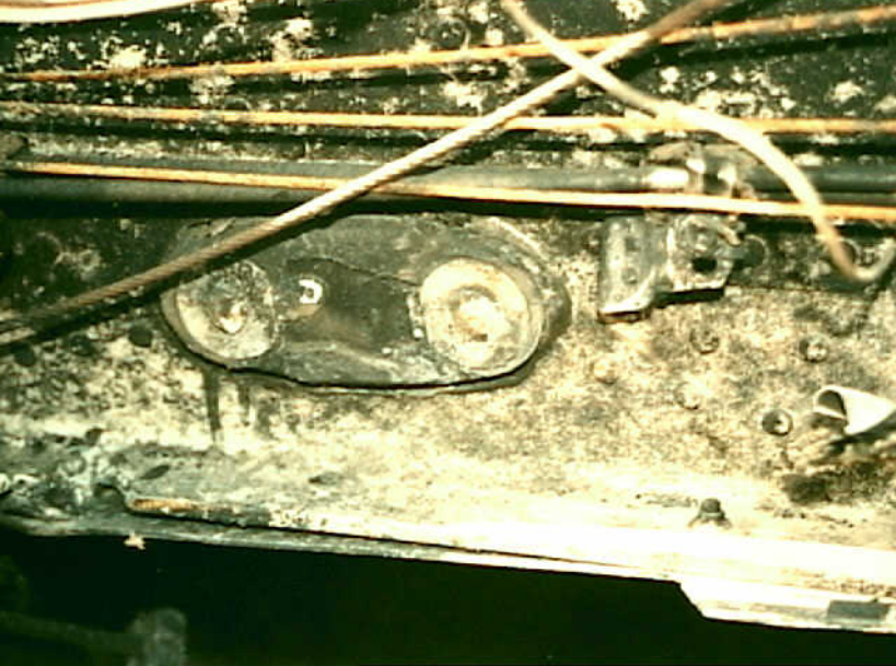
Structures 7 - Photo. 10 - View of the outboard attach fitting lower fasteners for the outboard flap hinge. Note: fasteners are sheared flush with spar.
