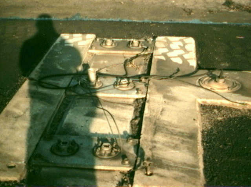
Structures 7 - Photo 8. View of damaged #55C runway sign mounting base
