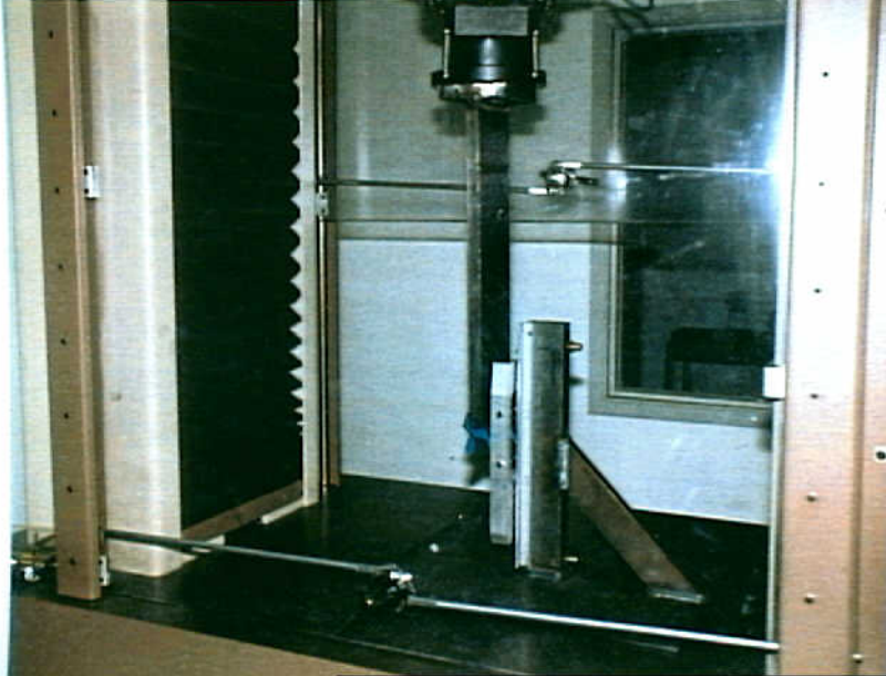
Structures 7 - Photo 3. Locking Pawl Assembly during Fully Locked Position Load Test
