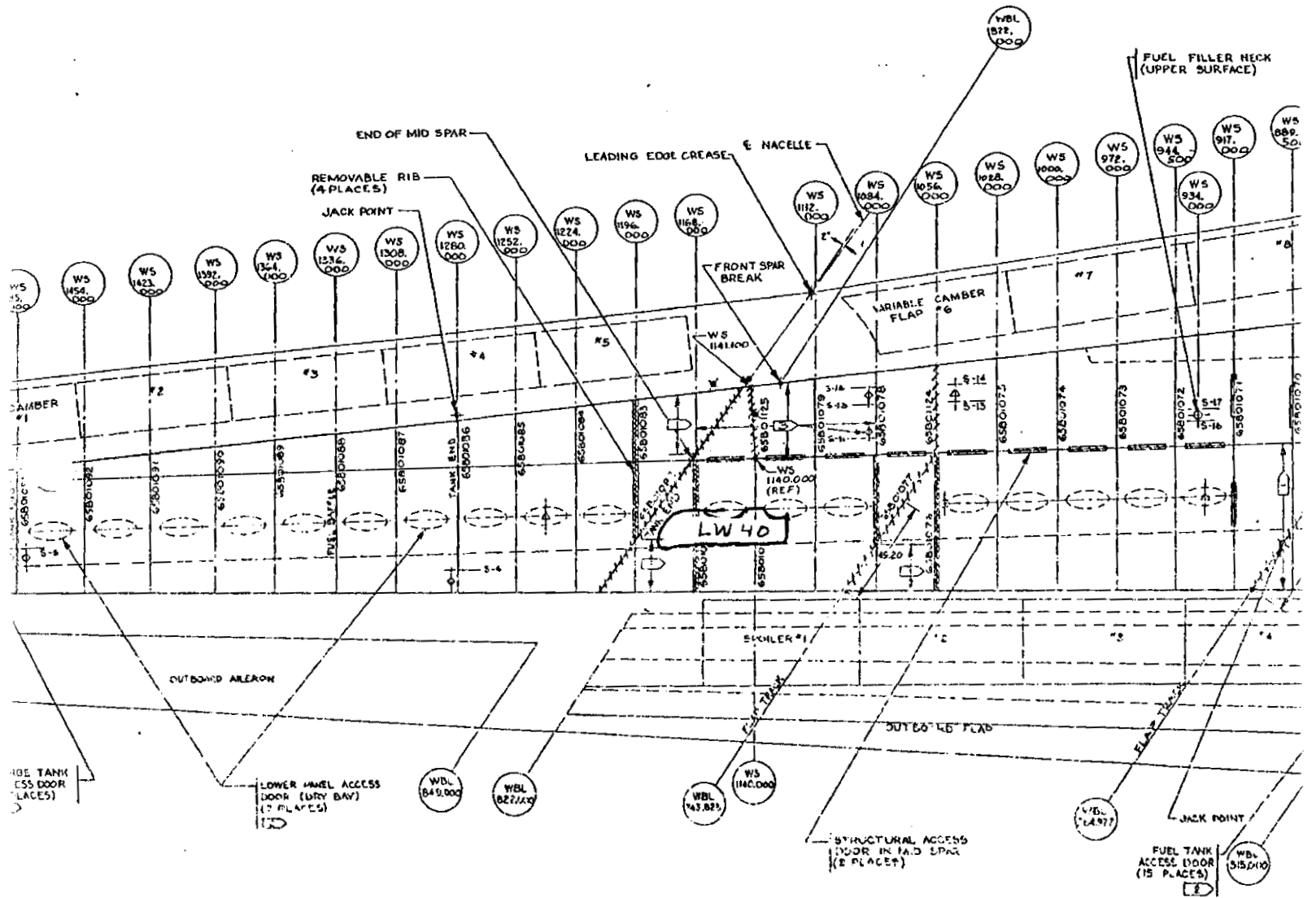
PLAN VIEW OF WING (NORMAL TO WING REF PLANE)
