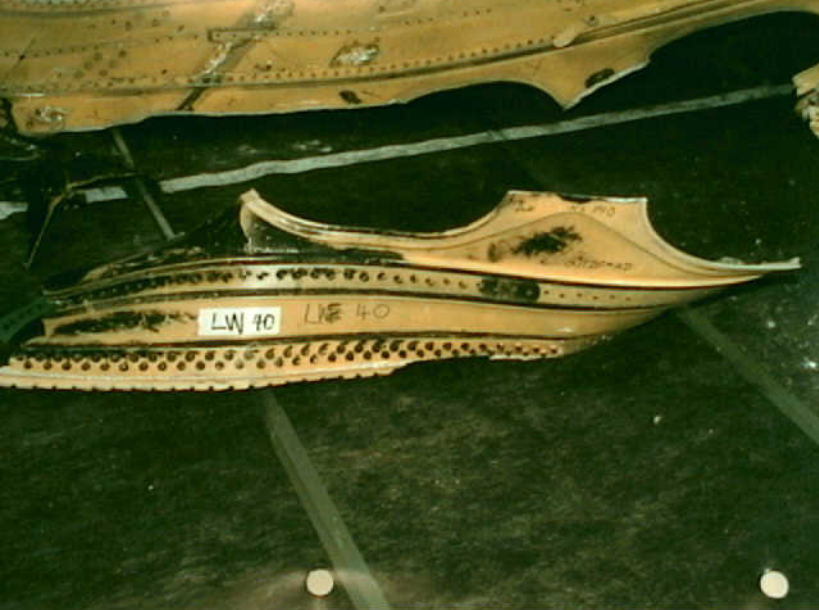
Structures 7 - LW-40 Photo 2
