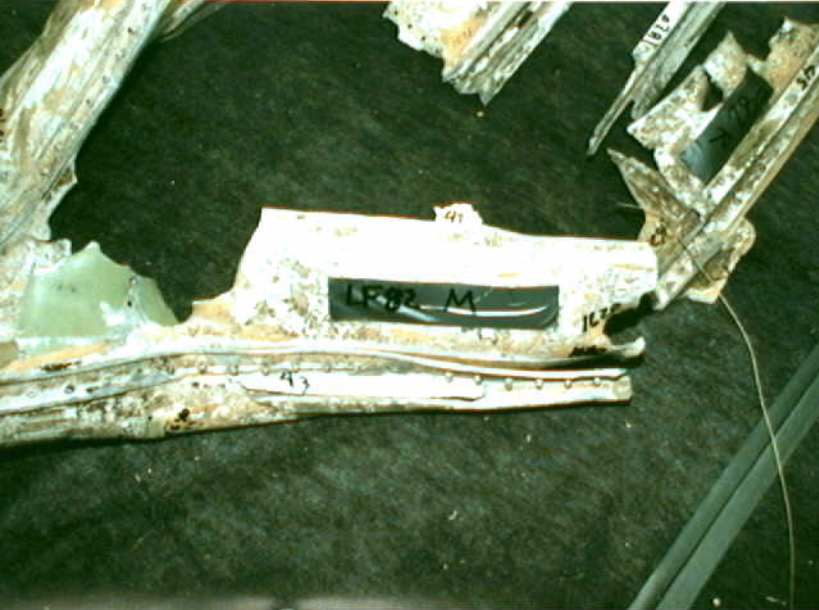
Structures 7 - LF82 - Photo 13
