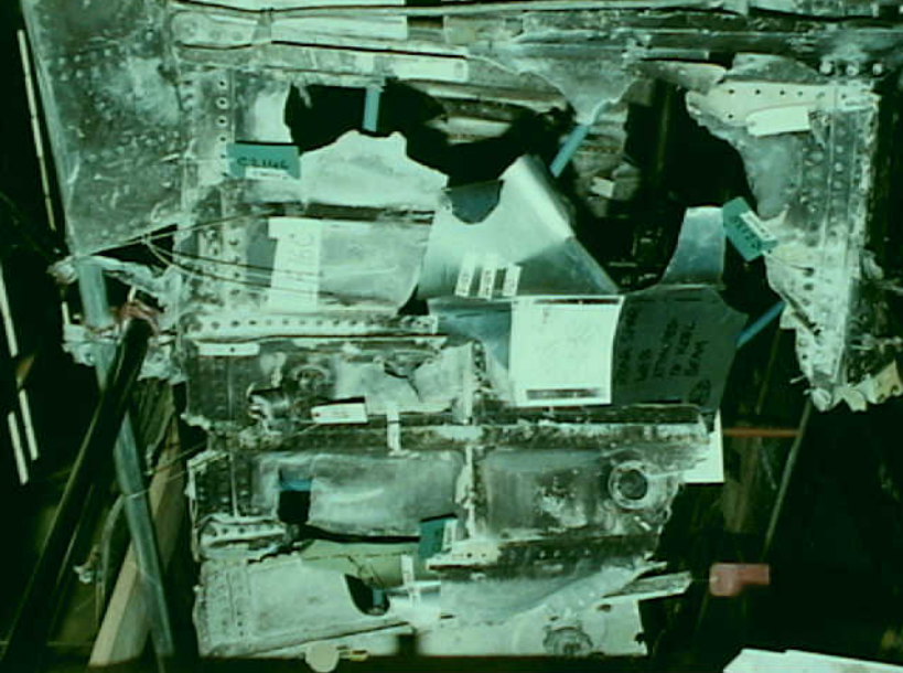
Structures 7 - LF16 - Photo 8
