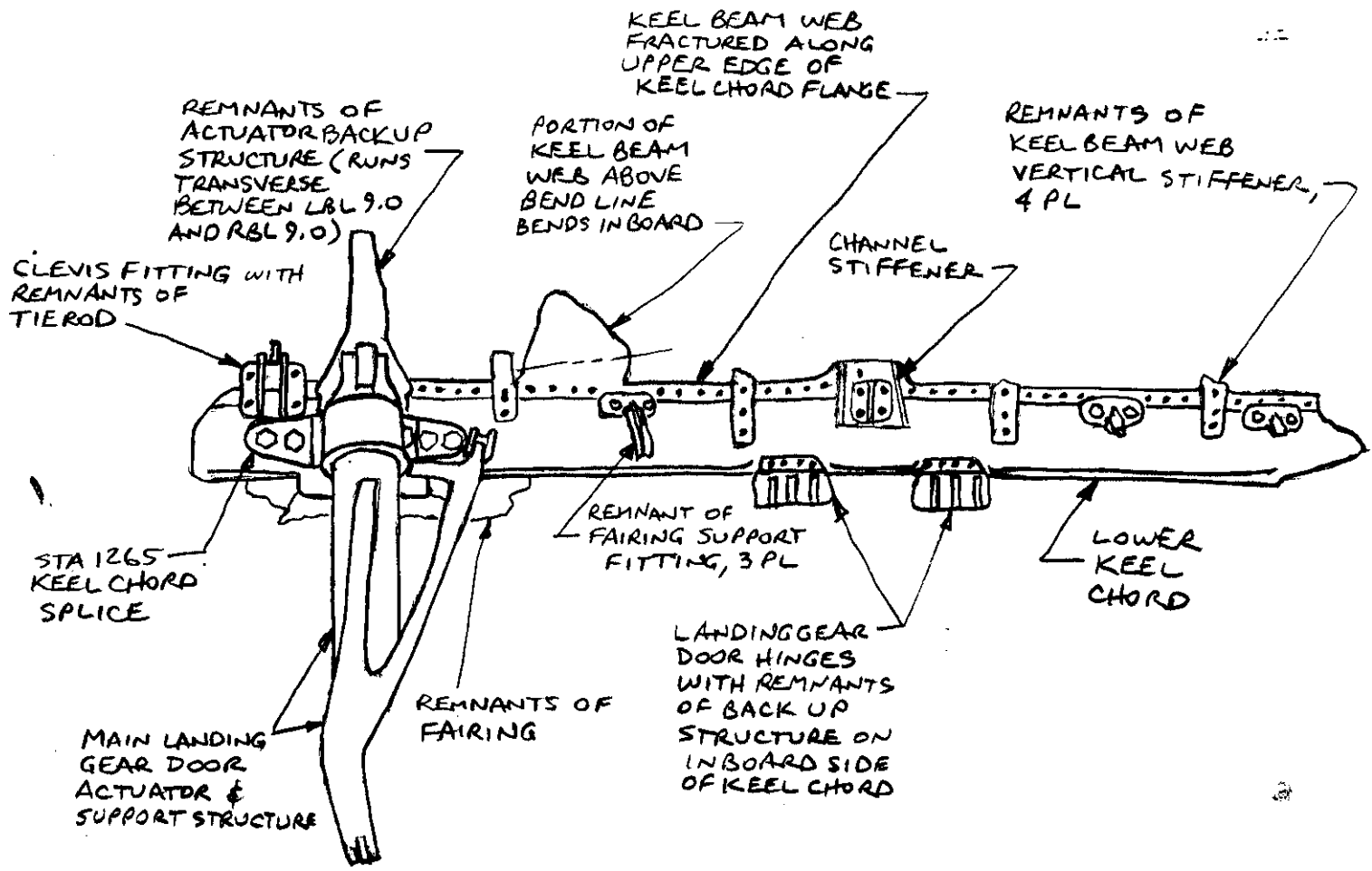
VIEW B-B LOOKING INBOARD
