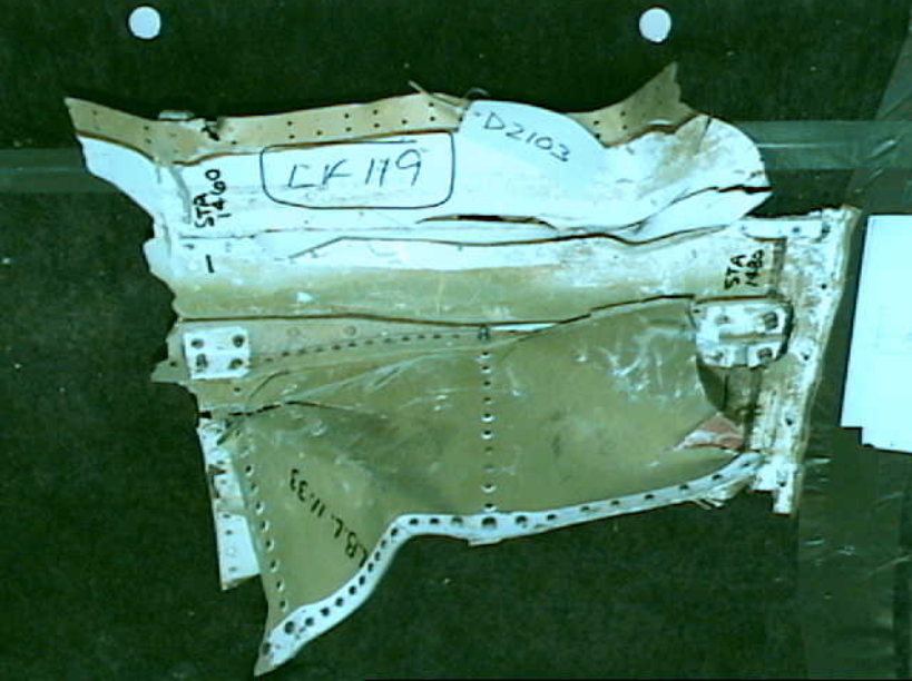
Structures 7 - LF119 - Photo 2
