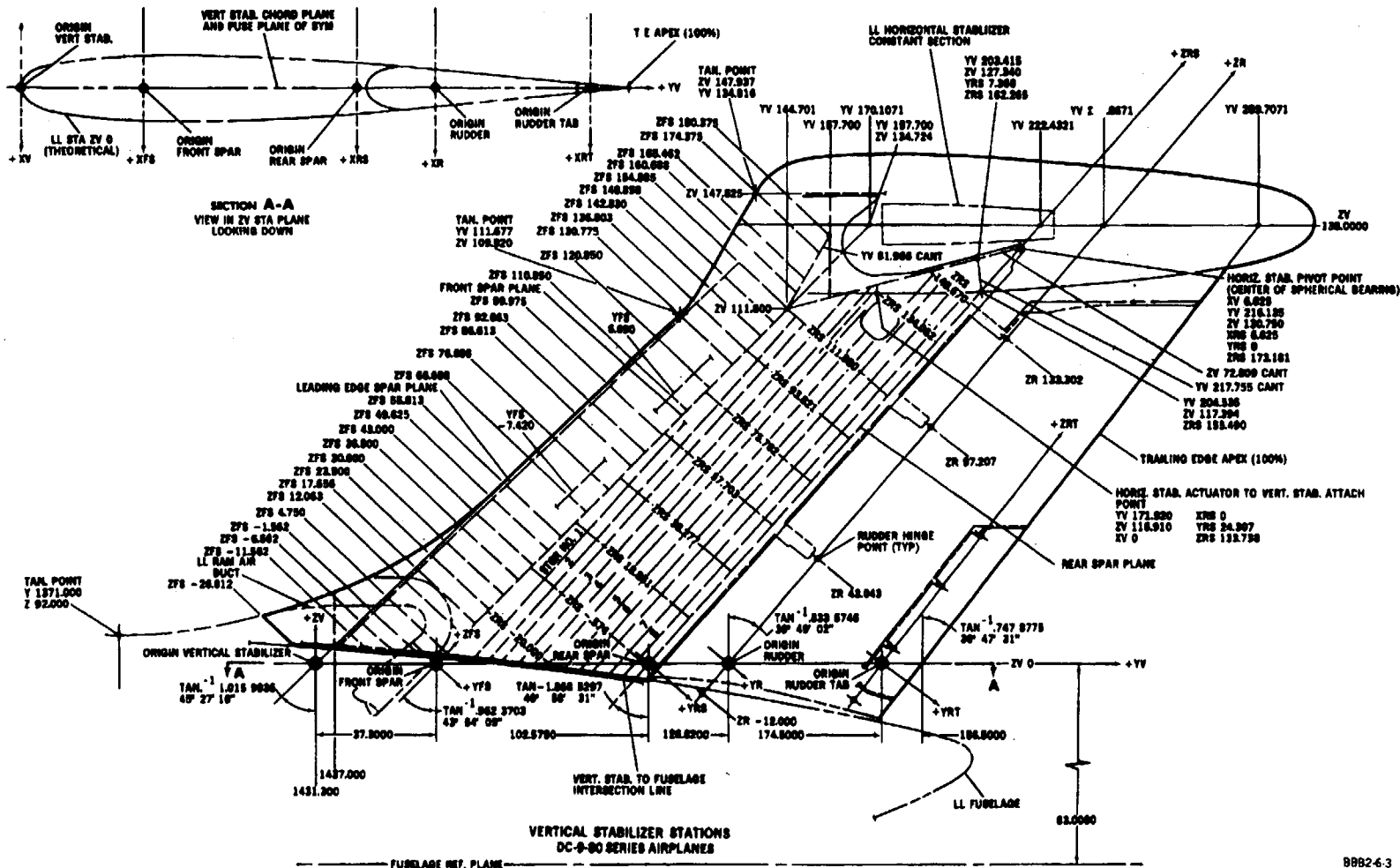
Vertical Stabilizer Station Diagram Figure 3
