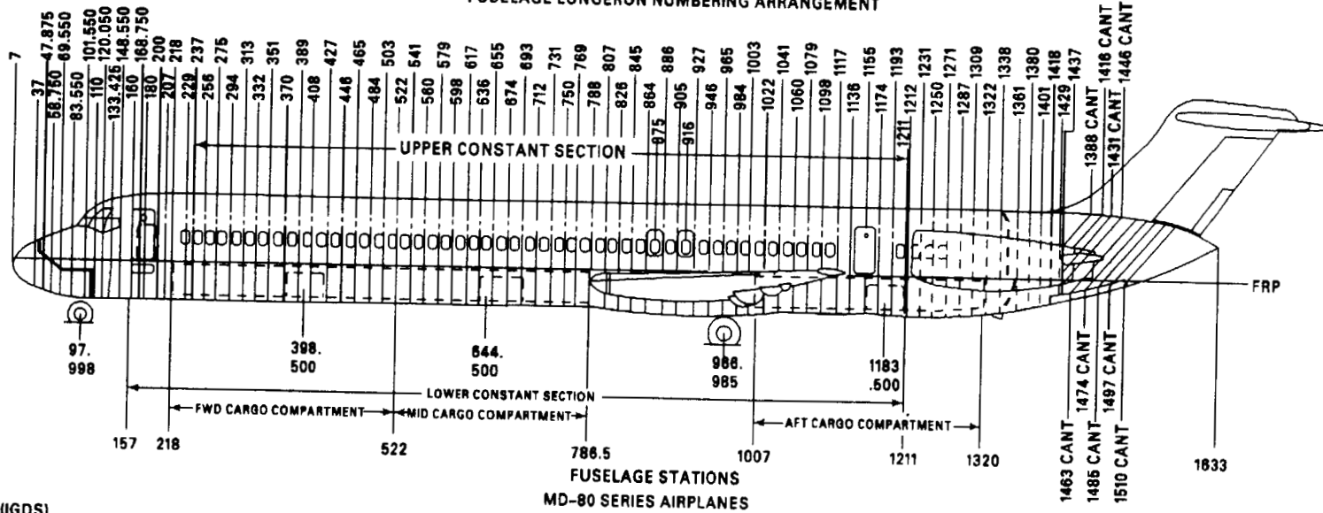
Fuselage Station Diagram Figure 1
