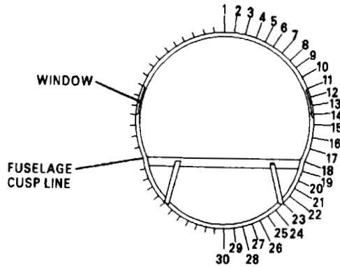
FUSELAGE LONGERON NUMBERING ARRANGEMENT
