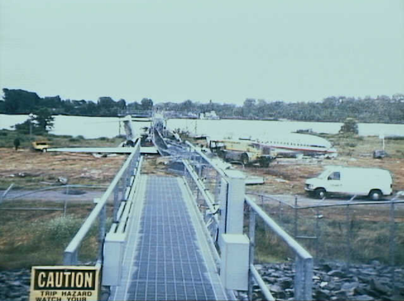
Structures 7 - Exhibit No. 7C - Photo 10. View of the damage to the forward fuselage, left side and crown. Note the approach lighting system structural support platform, entangled with the torn away airframe
