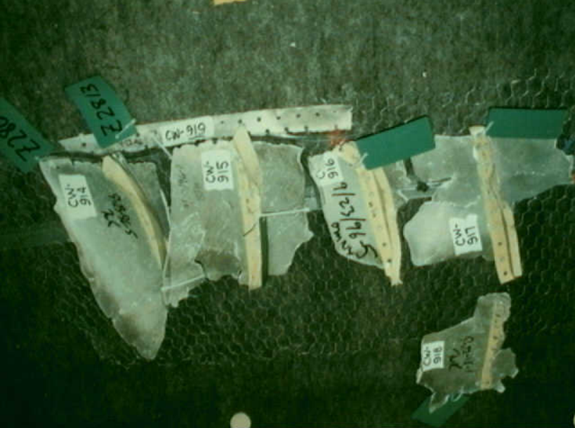
Structures 7 - CW-914 through CW-919 Photo 2
