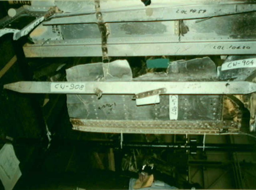
Structures 7 - CW-907 CW-908 Photo 1
