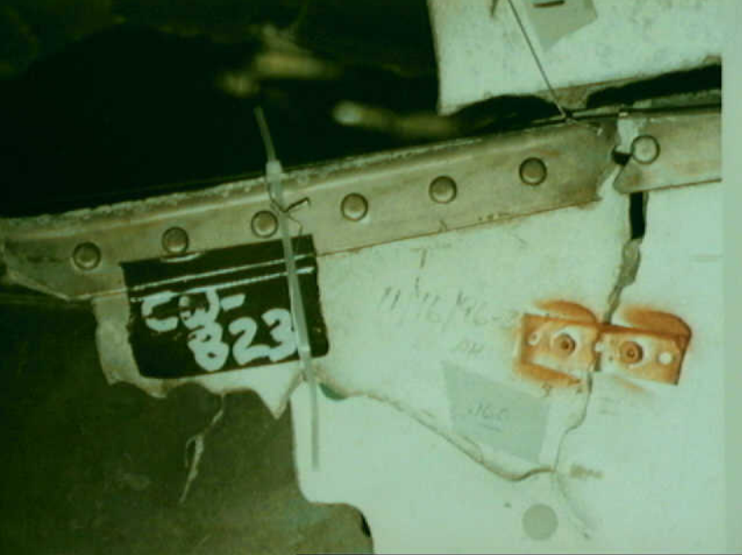
Structures 7 - CW-823 Photo 1
