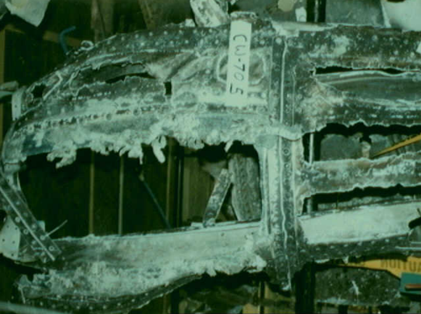
Structures 7 - CW-705 Photo 2
