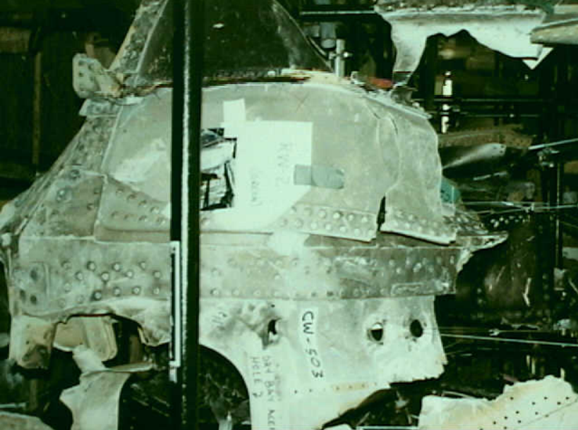
Structures 7 - CW-503 Photo 1
