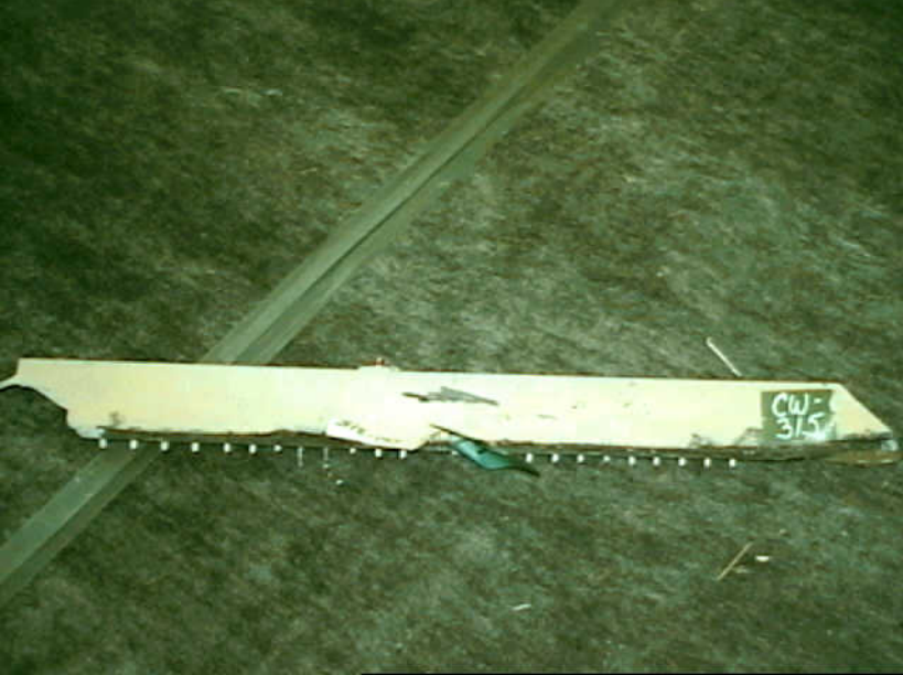
Structures 7 - CW-315 Photo 1
