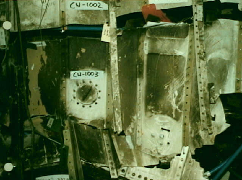
Structures 7 - CW-1003 Photo 4
