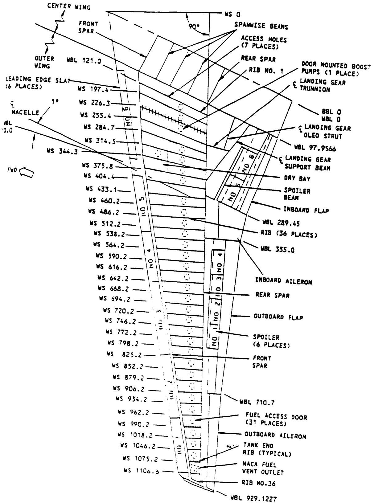
Figure 1. Wing Stations
