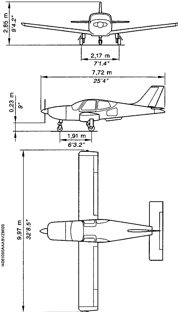
Figure 1.21A – THREE VIEW DRAWING
