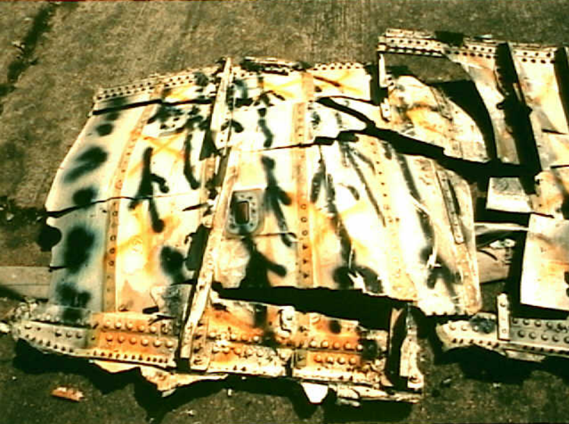
Sequencing Group 18 - Appendix B - Photo 16. Deformation of rear spar.
