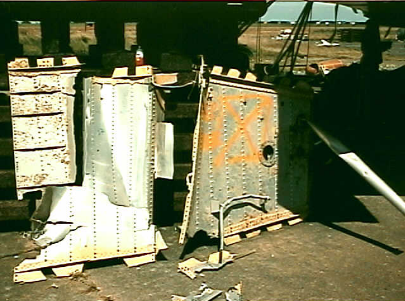
Sequencing Group 18 - Appendix B - Photo 15. Deformation and damage of B.L.O rib.
