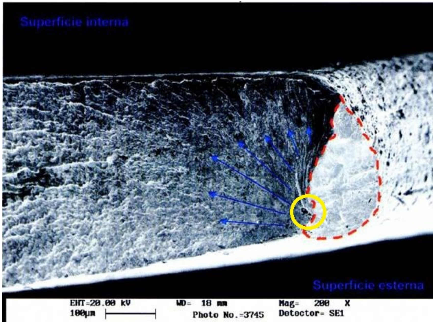
Photo 2 – Close view, microscopic image of crack propagation (Courtesy of Leonardo)
