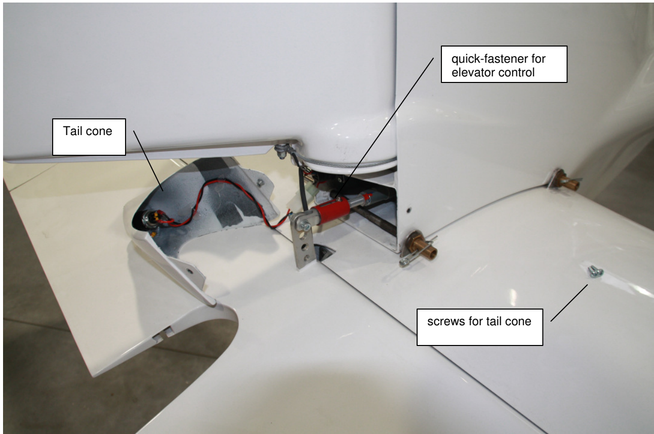
Figure 6 – elevator quick-fastener
