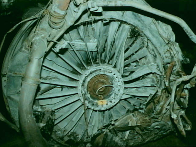
Powerplants 8. Photo 8. Number 3 Engine Side View
