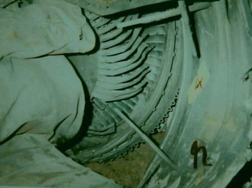
Powerplants 8. Photo 13. Number 4 Engine Rear View
