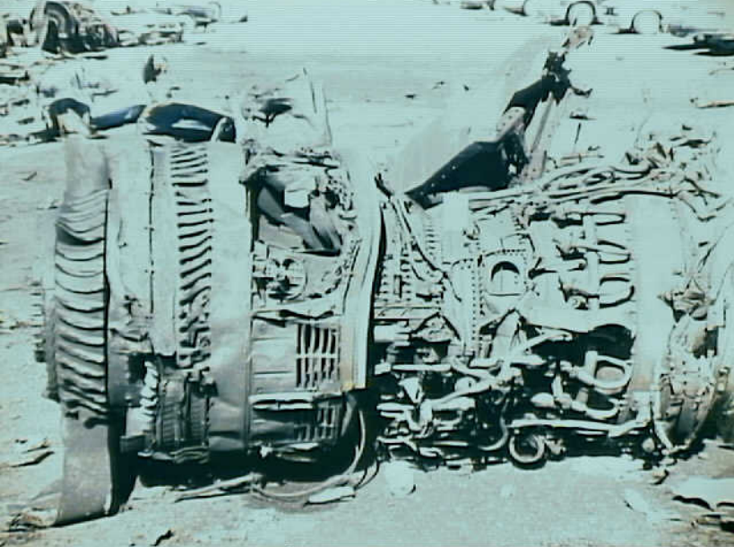
Powerplants 8 - Photo 9. side view of No. 2 engine.
