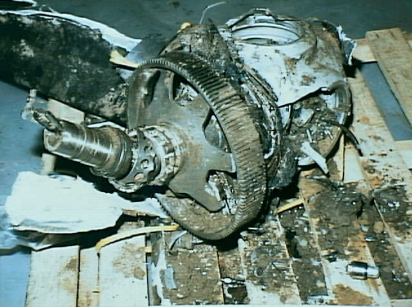
Powerplants 8 - Photo 9. Left propeller servo piston
