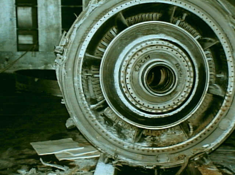
Powerplants 8 - Photo 9. Engine No. 1 front of HPC
