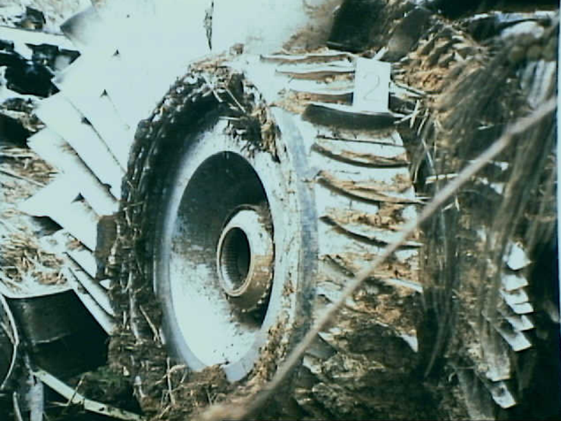
Powerplants 8 - Photo 8. No. 2 engine fan
