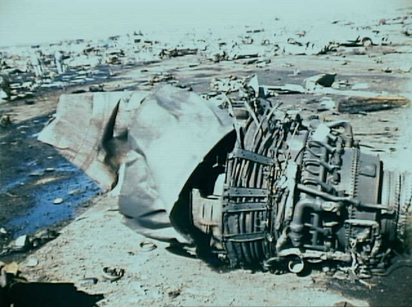
Powerplants 8 - Photo 6. Side view of No. 1 engine.
