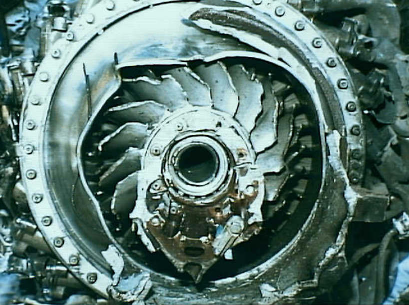
Powerplants 8 - Photo 6. Right engine low pressure impeller leading edge
