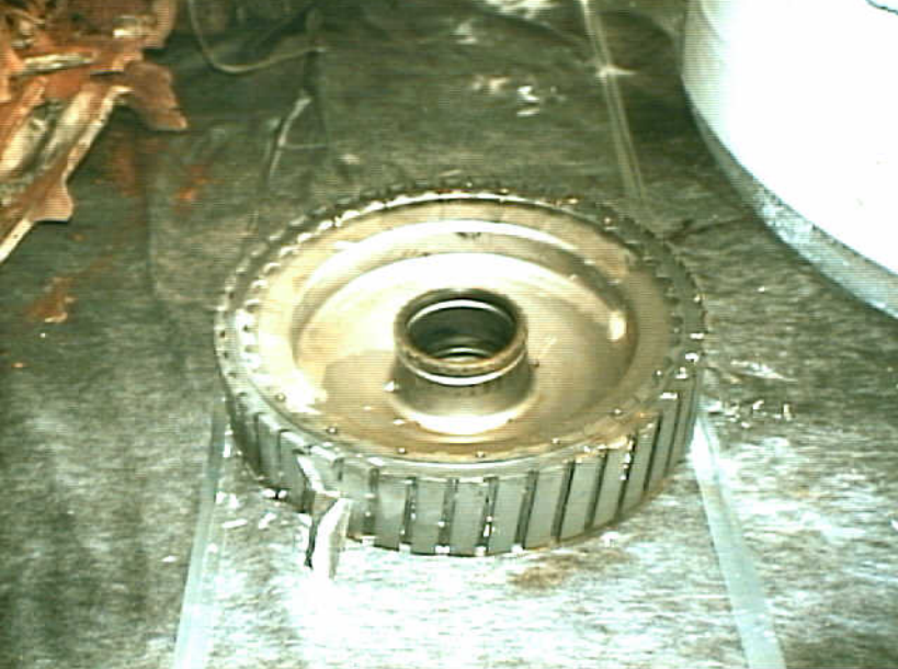
Powerplants 8 - Photo 6. Engine No. 1, fan hub.
