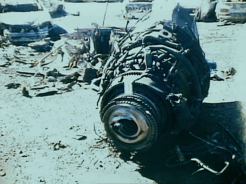
Powerplants 8 - Photo 5. Front view of No. 1 engine showing HPC disks.
