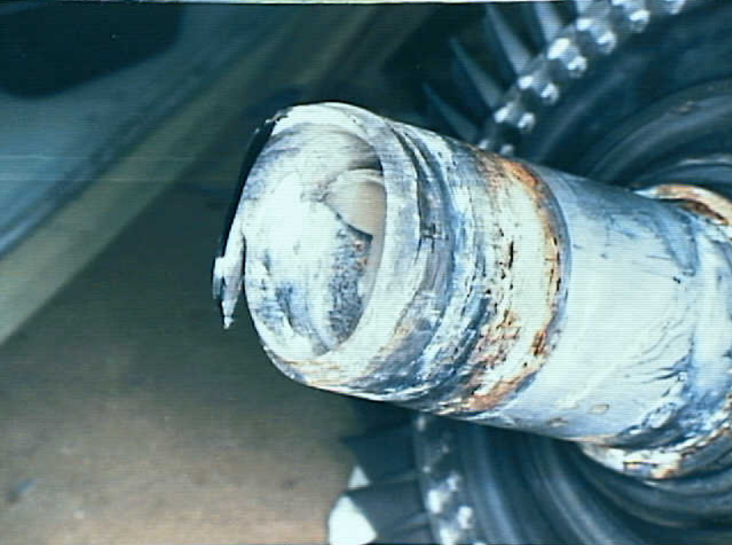
Powerplants 8 - Photo 49. Fractured low pressure and power turbine shafts from right engine
