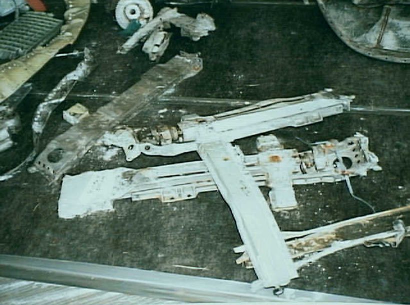
Powerplants 8 - Photo 48. Thrust reverser actuators.
