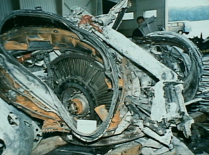
Powerplants 8 - Photo 47. Engine No. 4, rear, showing fifth stage turbine hub and blades and sixth stage turbine disk and blades.
