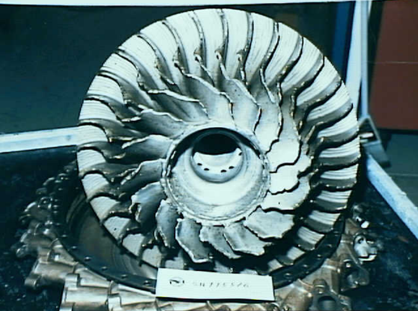
Powerplants 8 - Photo 46. Right engine low pressure impeller
