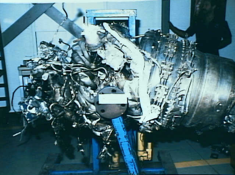
Powerplants 8 - Photo 45. Right engine as received at Pratt & Whitney of Canada
