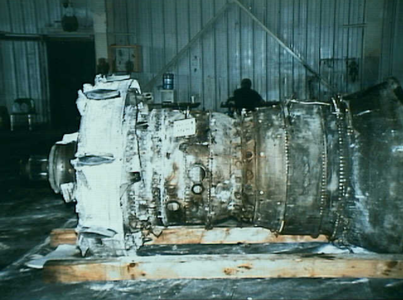
Powerplants 8 - Photo 45. Engine No. 4, top
