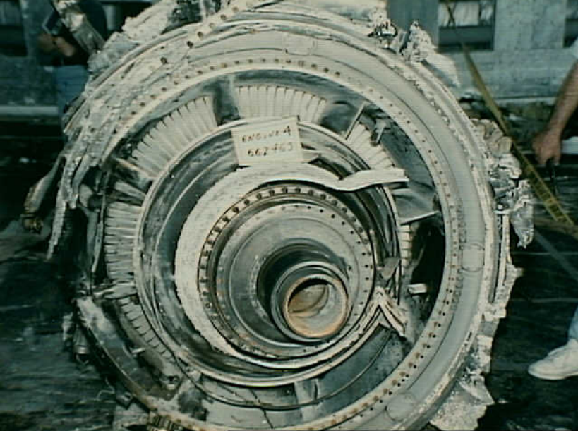
Powerplants 8 - Photo 44. Engine No. 4, front of HPC
