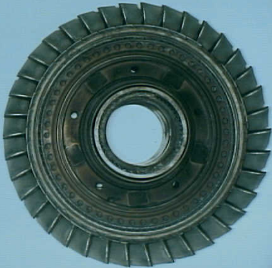
Powerplants 8 - Photo 38. Left engine high pressure turbine disk and blades
