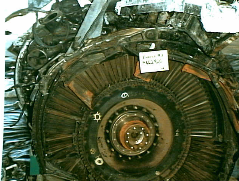
Powerplants 8 - Photo 37. Engine No. 3, rear, showing fifth stage turbine hub and blades and sixth stage turbine disk and blades.
