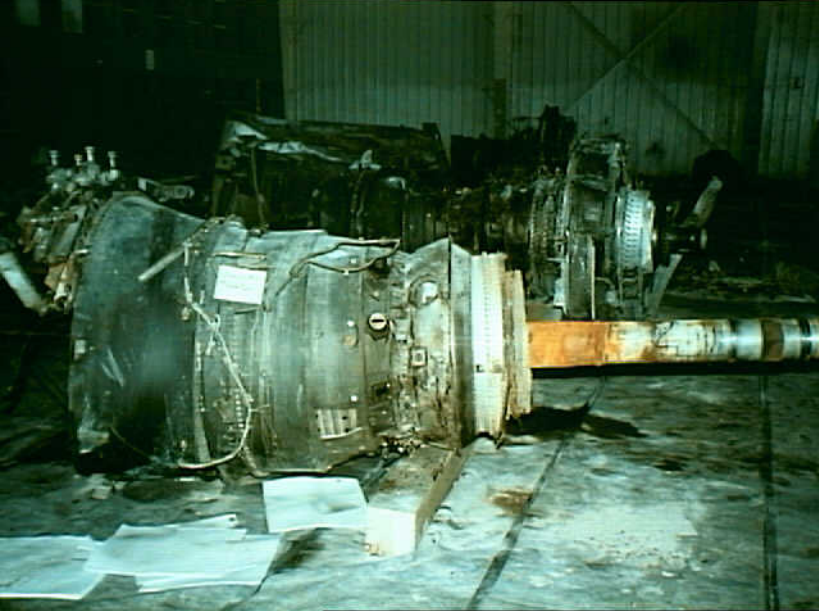
Powerplants 8 - Photo 35. Engine No. 3, HPC, right side, and LPT shaft
