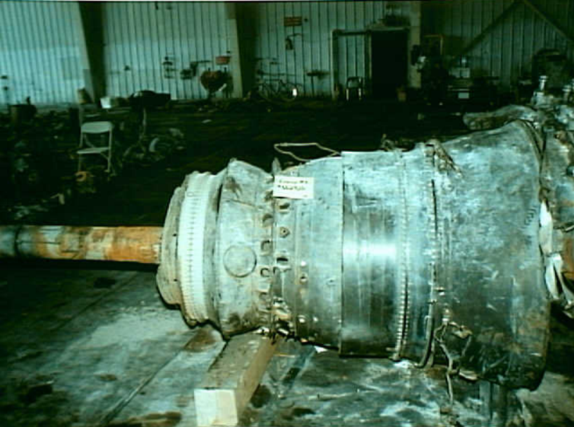
Powerplants 8 - Photo 34. Engine No. 3, HPC, left side, and LPT shaft.
