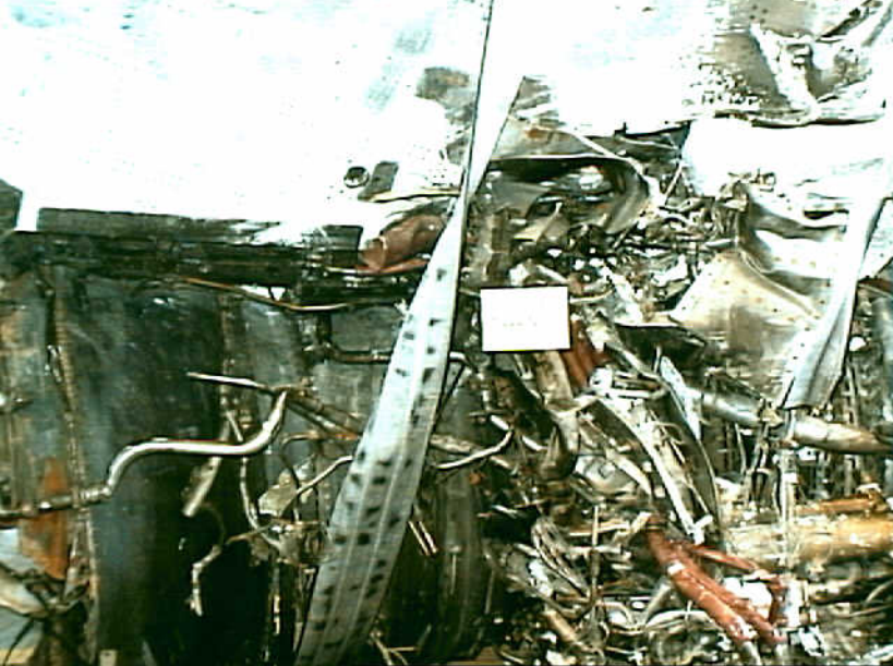
Powerplants 8 - Photo 33. Engine No. 3, right side and pylon.
